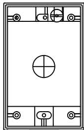
ALUMINUM RECEPTACLE BOX 2 3/4" X 4 5/8" X 2 3/8" DEEP
