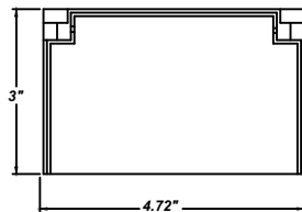
HORIZONTAL GFI COVER PLATE
