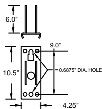
S42 BASE PLATE
