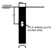
BELOW GRADE SECTION OVALIZED, POWDERCOATED, AND RUBBER PIPE WRAPPED
